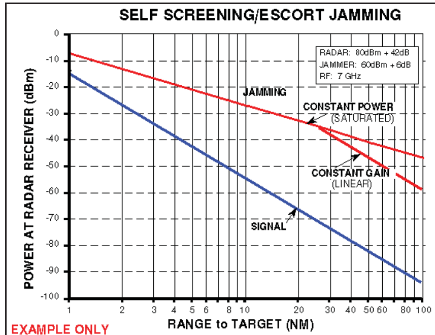
Figure 1. Sample Constant Gain / Constant Power Graph.
