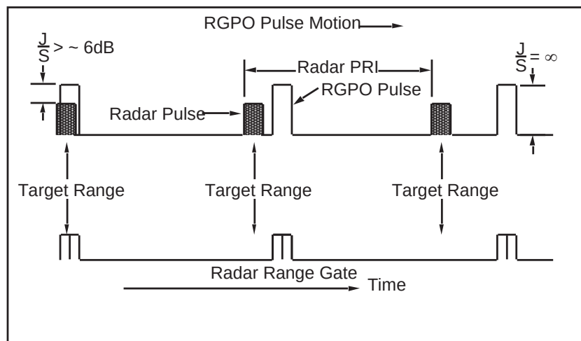
Figure 6. Range Gate Pull Off.
