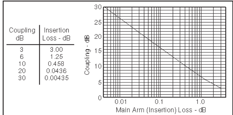
Figure 2. Coupling Insertion Loss.
