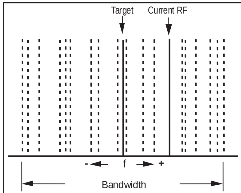
Figure 13. Velocity Noise.
