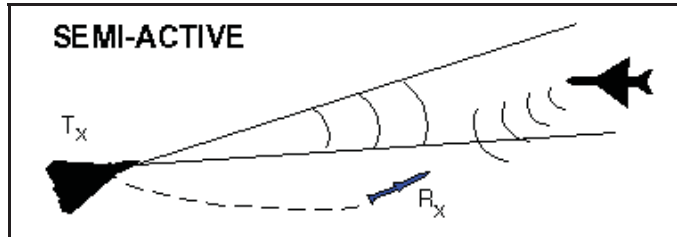
Figure 5. Bistatic Radar.
