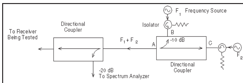
Figure 1. Receiver Test Setup When Antenna Can Be Removed.
