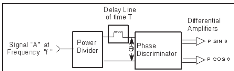
Figure 2. Frequency Discriminator.
