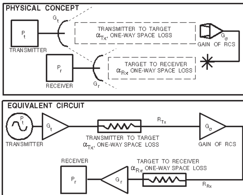
Figure 1. Bistatic Radar Visualized.
