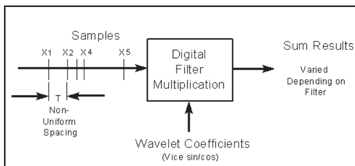
Figure 7. Wavelet Filtering.
