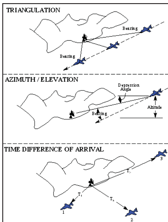
Figure 3. Passive Emitter Location Techniques.
