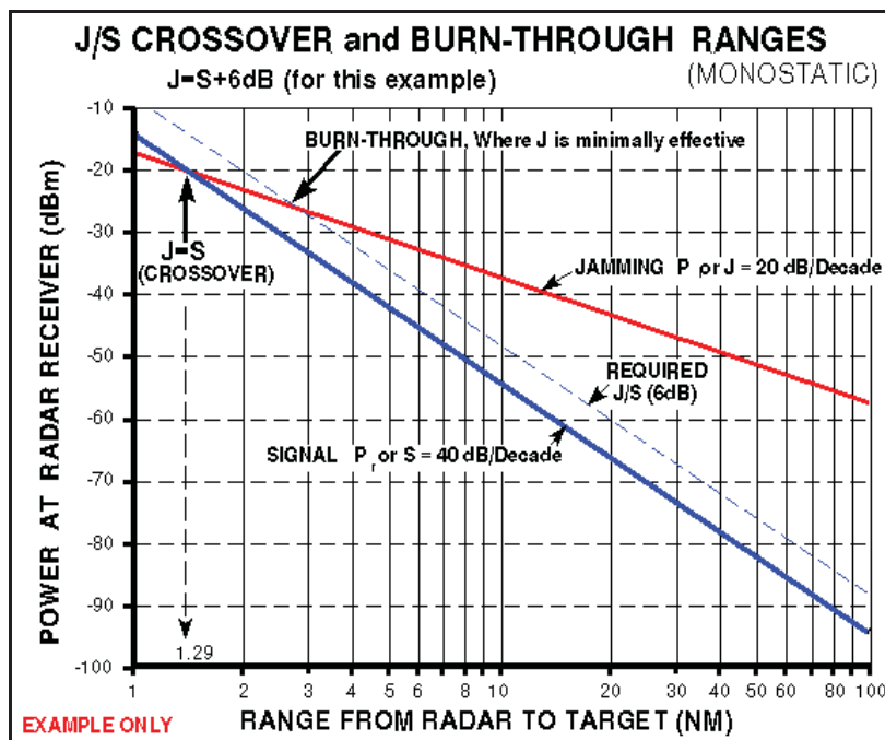
Figure 1. Sample J and S Graph.
