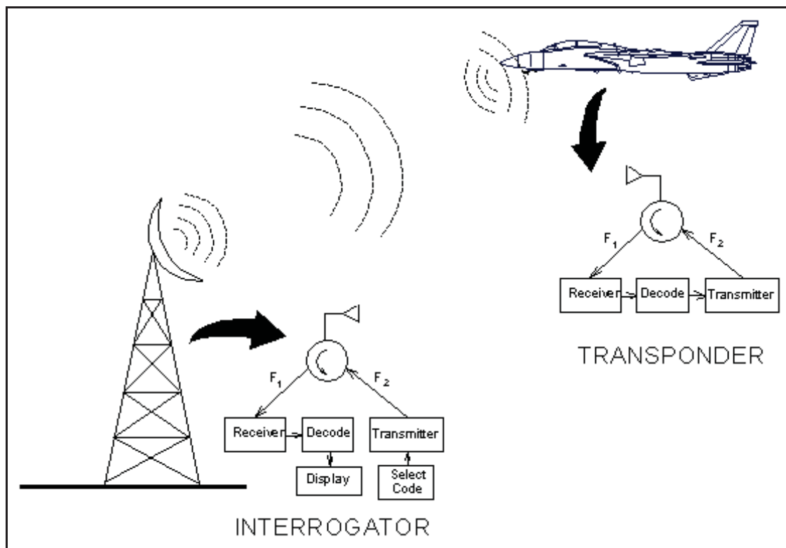
Figure 1. IFF Transponder.
