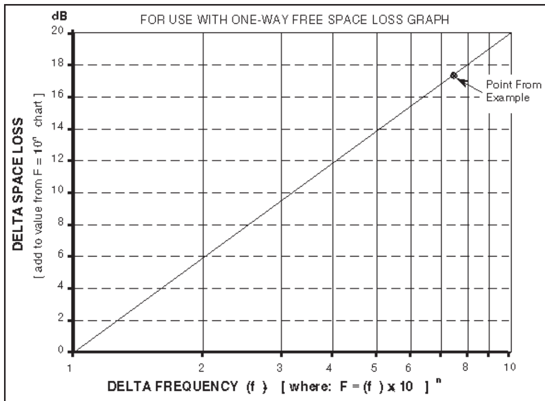
Figure 5. Frequency Extrapolation.
