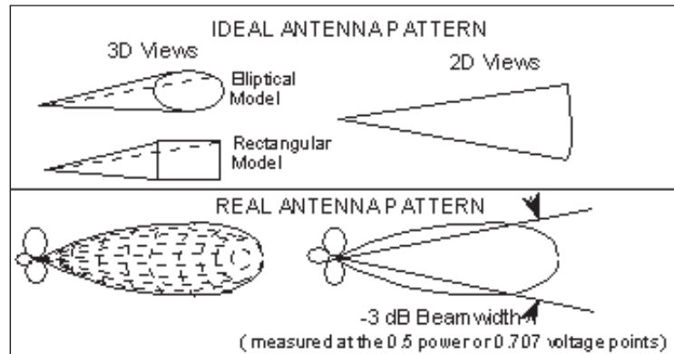
Figure 3. Antenna Beamwidth.
