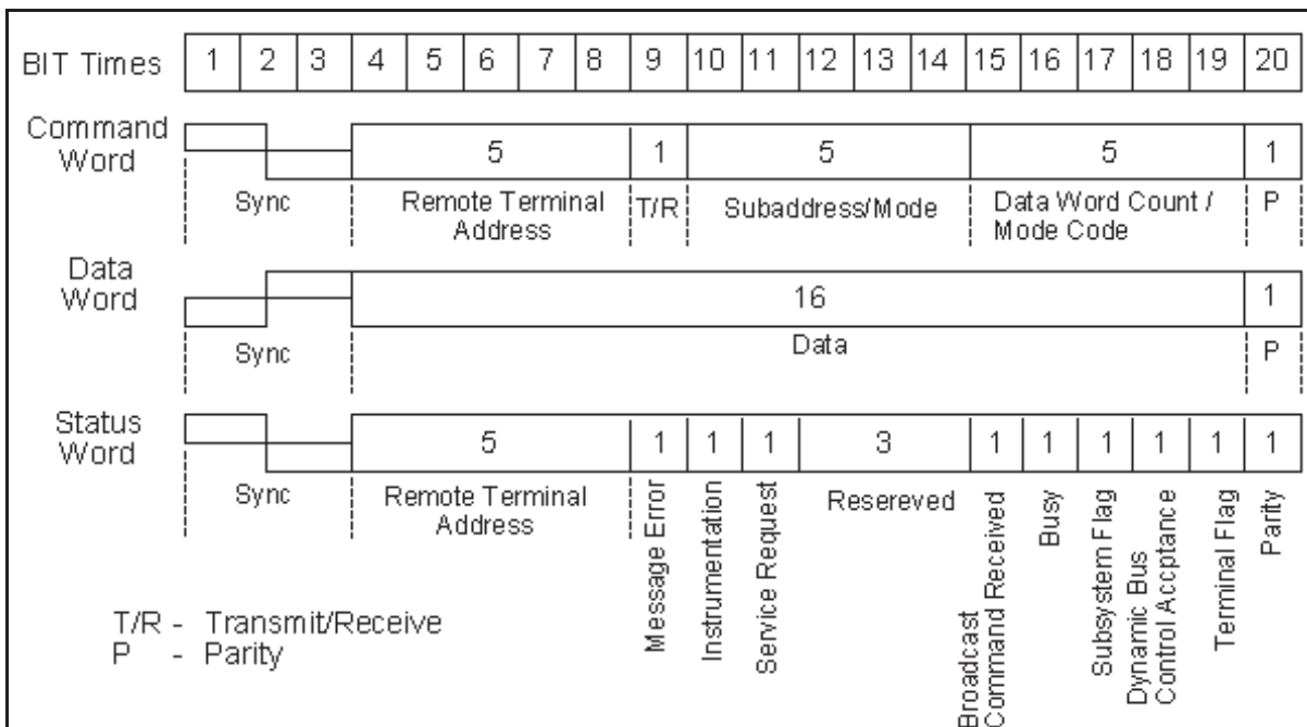
Figure 3. 1553 Word Formats.
