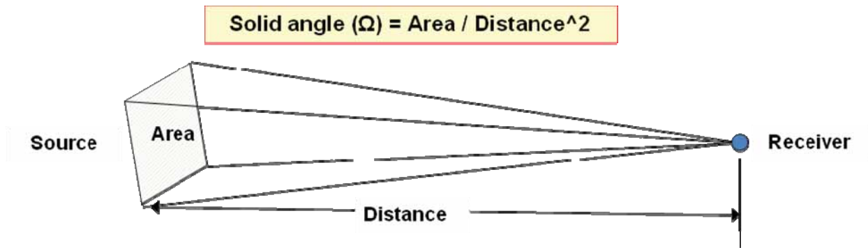
Figure 3. Solid Angle.
