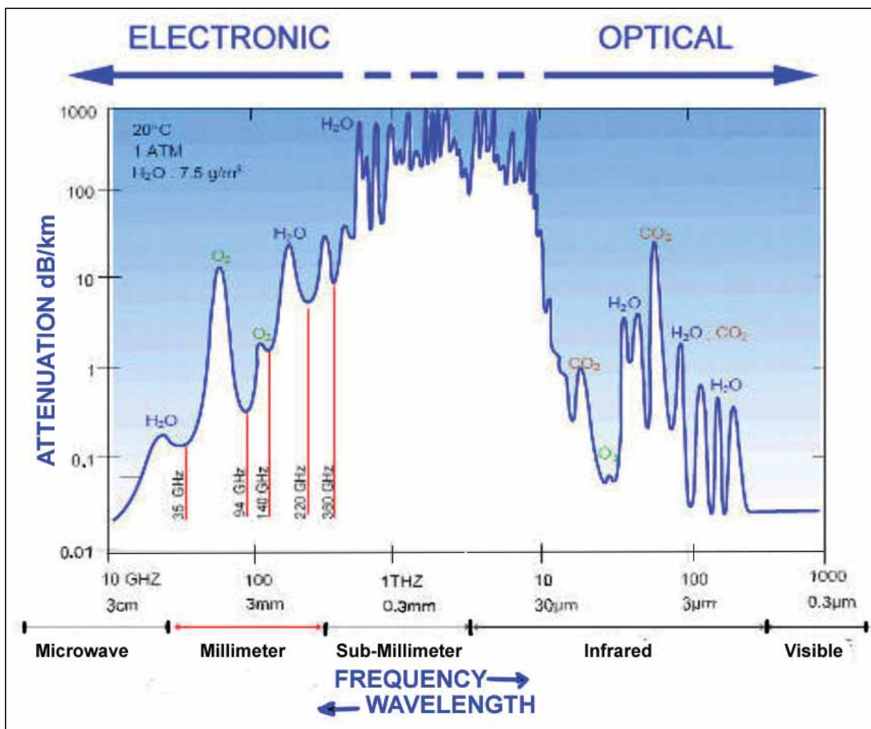
Figure 1. Atmospheric Absorption of Millimeter Waves.
