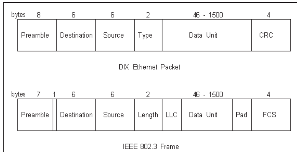
Figure 1. Ethernet Frame.
