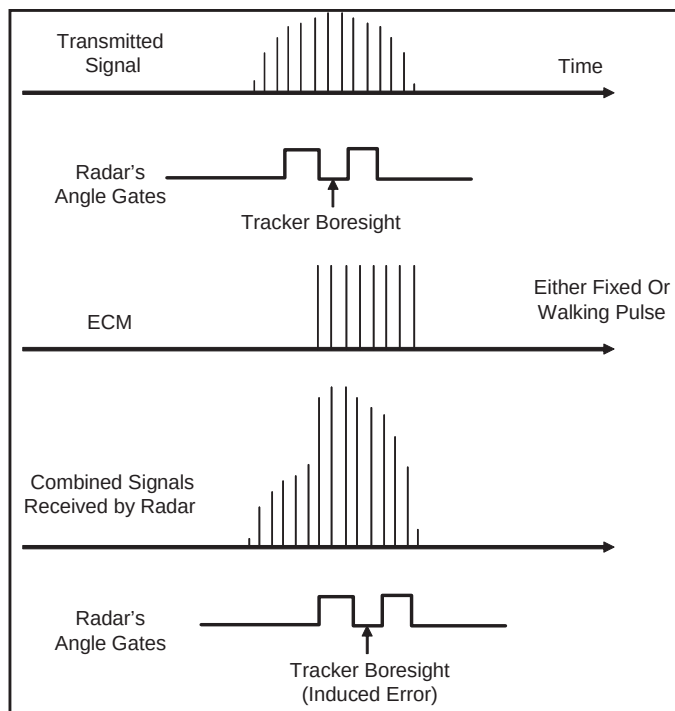
Figure 10. TWS Jamming.
