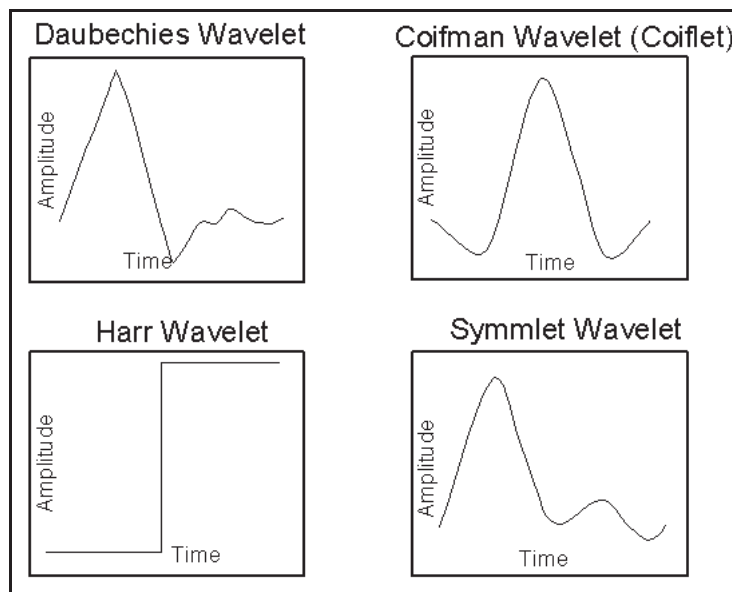
Figure 8. Sample Wavelet Functions.
