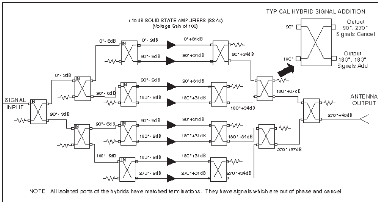
Figure 6. Combiner Network.
